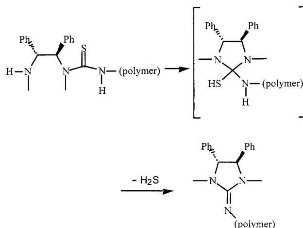
Scheme 4. Guanidine formation during polymerisation
