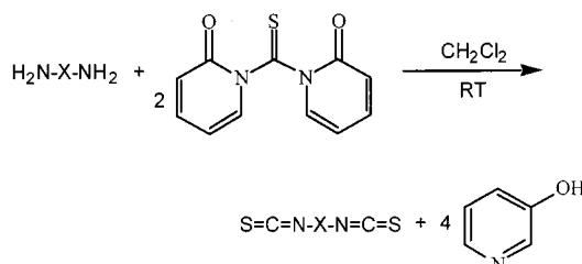
Scheme 2. Synthesis of isothiocyanates from primary amines and 1,1'-thiocarbonylbis(2,2'-pyridone)
