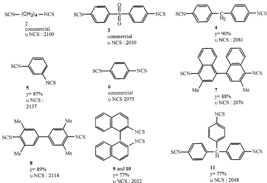
Scheme 3. Yields and NCS bands of the isothiocyanates synthesized
