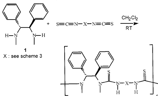
Scheme 1. Preparation of polythioureas from (1 R ,2 R )-(+)- N,N' -dimethyl-1,2-diphenylethylenediamine and diisothiocyanates
